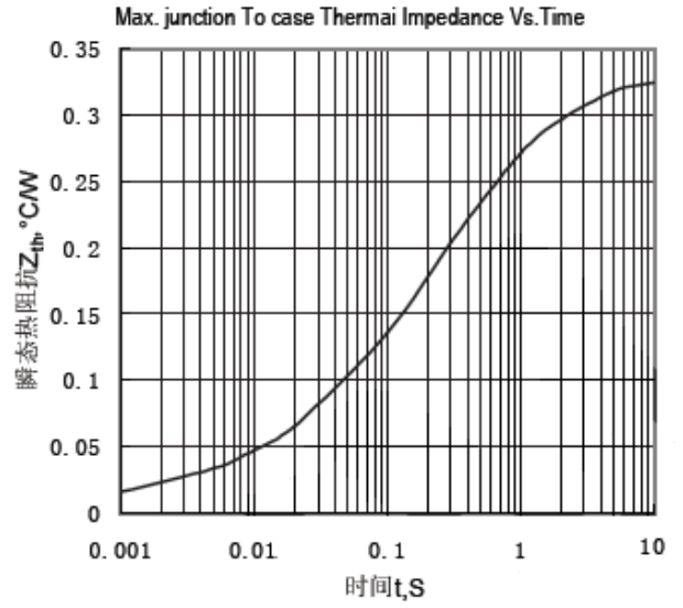
Fig.2 结至管壳瞬 热阻抗
